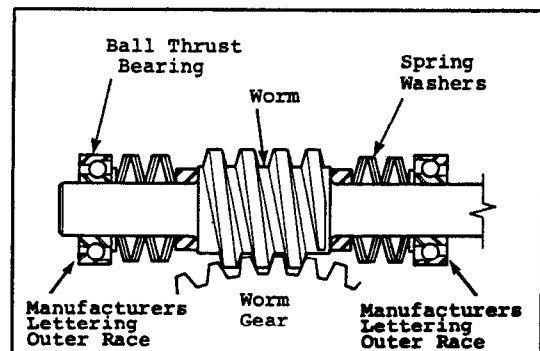
Worm Bearing Orientation
